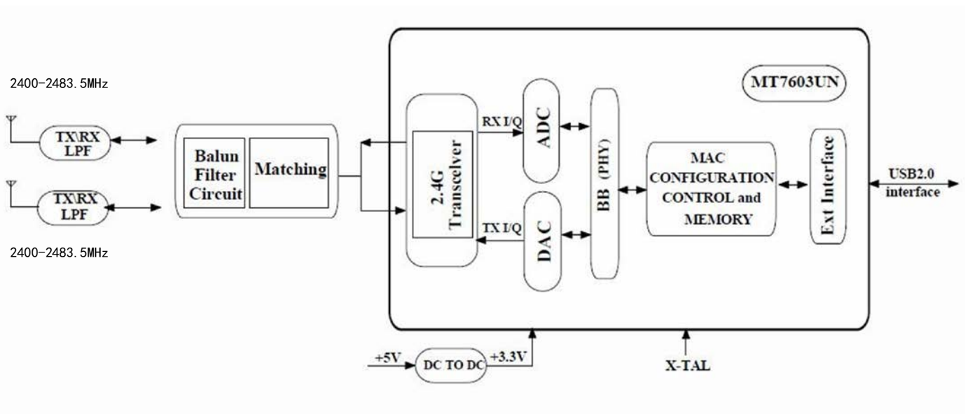
Figure 1-1 WDN221M block diagram and SystemInterface
